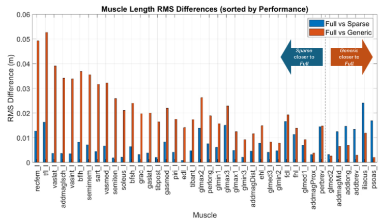
Figure 1. A) Representation of the workflow for creating personalized models based on sparse medical images: CLinically Informed Model Builder (CLIMB) . B) Exemplary waveforms of muscle length over gait cycle for rectus femoris muscle for the three models Full (black), Sparse (blue) and Generic (red). C) Muscle length RMSD over gait cycle per muscle.
