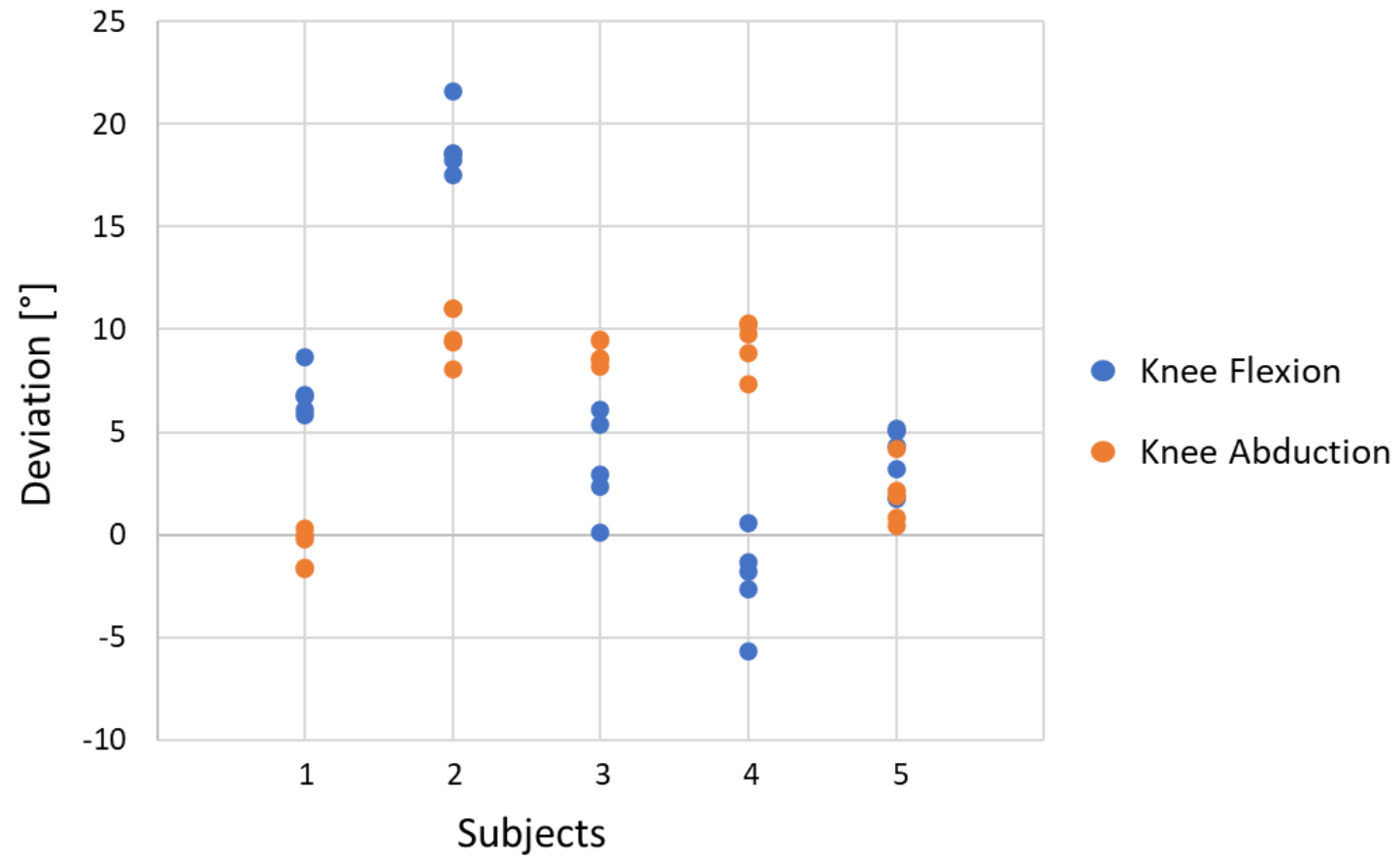
Figure 1. Deviation in degrees ( ^{\circ} ) of knee flexion (blue) and knee abduction (orange) angle between IMU and OMC. Positive values indicate a higher IMU angle. Each dot represents one 180^{\circ} COD trial.
