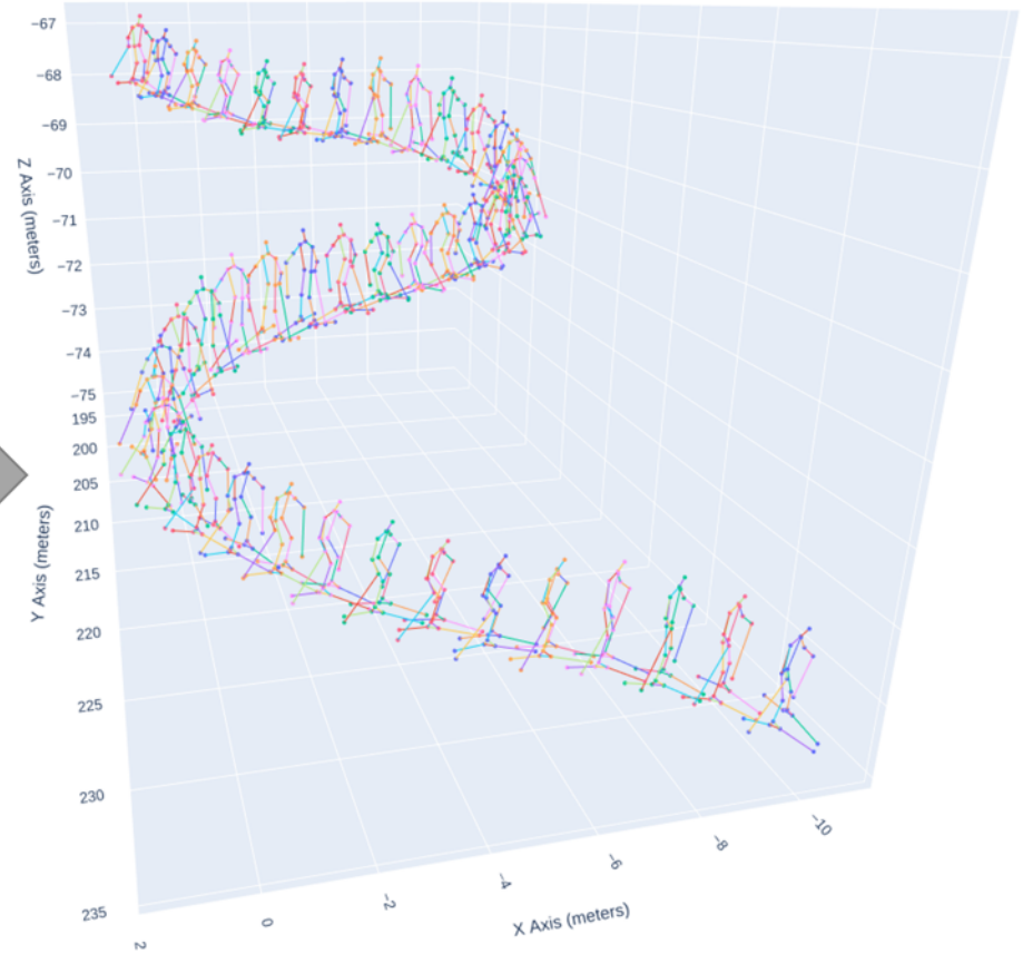
Figure 1. Left: Sample visualizations of keypoint detection results using our ski-specific model on various perspectives. Right: 3D kinematic reconstruction of a skier's run, derived from the keypoints detected in a series of images as shown the left.
