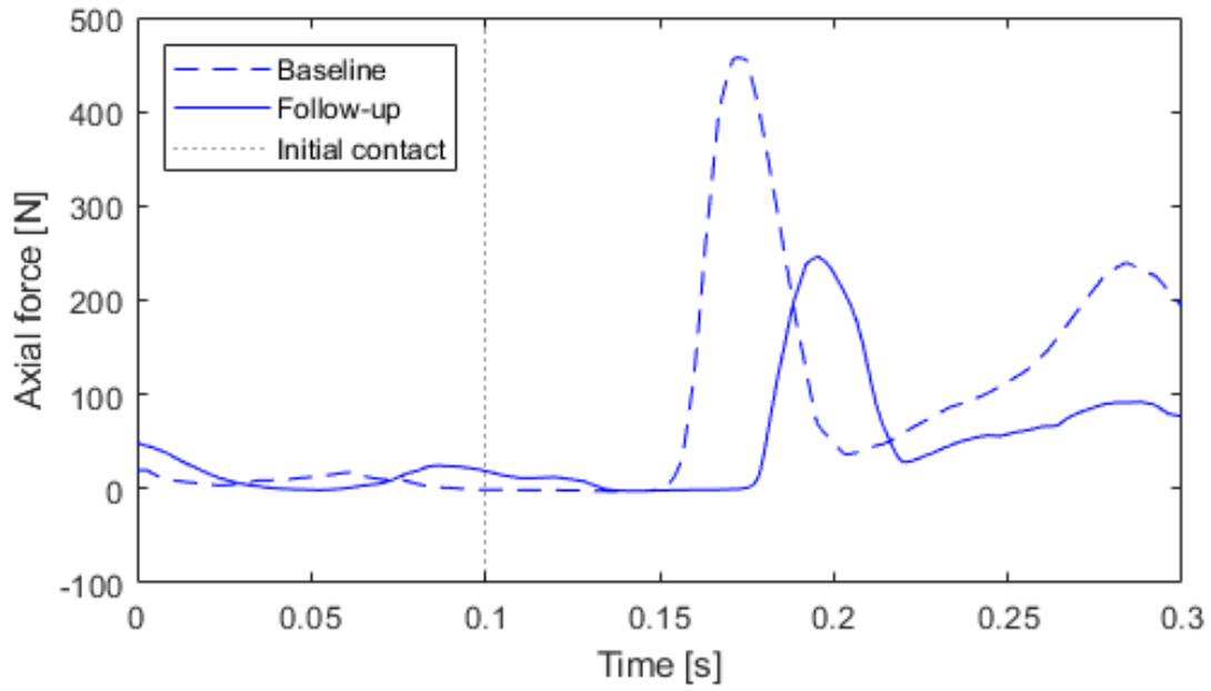
ACL forces during COD, before (Baseline) and after (Follow-up) an 8-week injury prevention exercise program. The x-axis describes the time range of the COD, defined as 100 ms before and 200 ms after initial contact (ground reaction force greater than 20 N).
