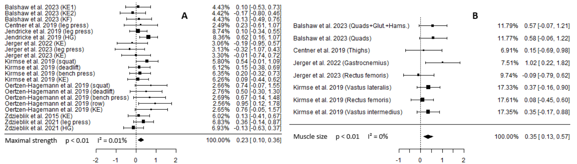
Figure 1: A) Maximal strength and B) Muscle size estimates. KE = knee extension, KF = knee flexion, HG = handgrip.
